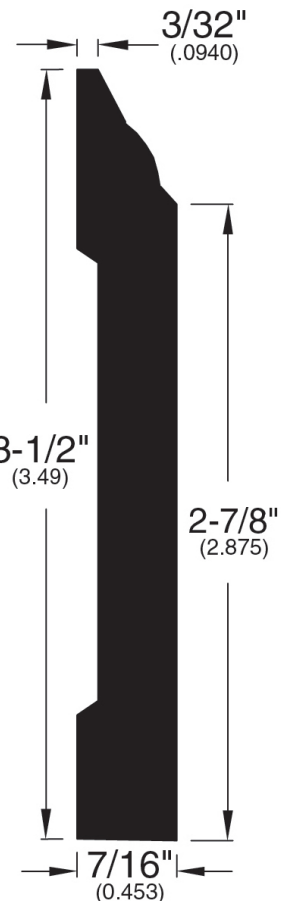
Wall Base (003)
