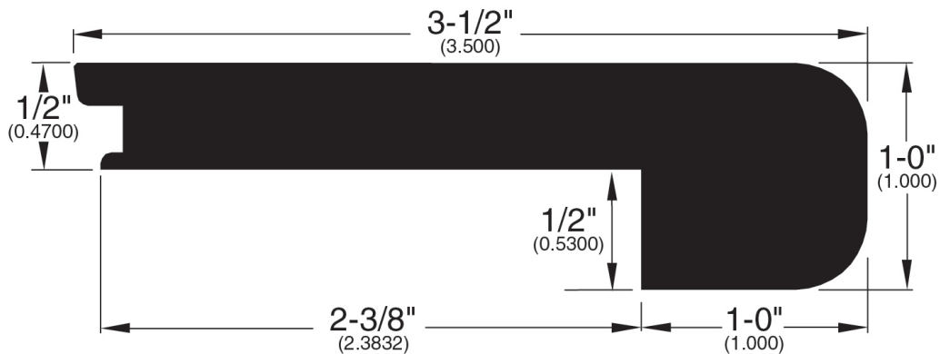
Stair Nose (219)
