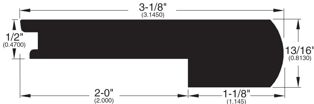
Stair Nose (012)
