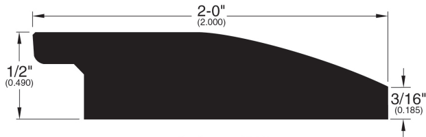
Reducer (066)
