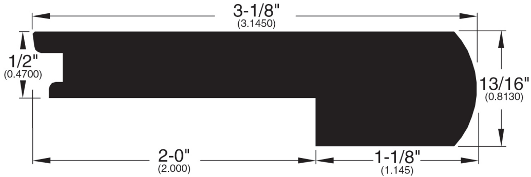
Stair Nose (012)
