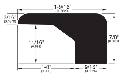
Square Nose (027)
