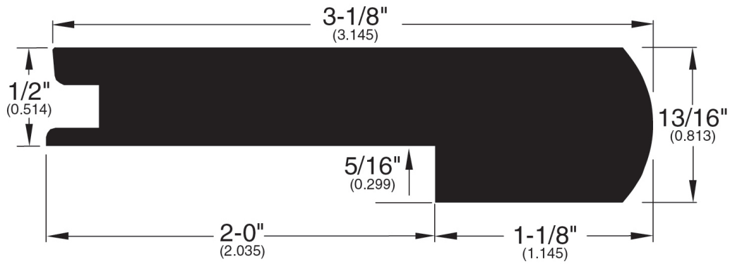
Stair Nose (091)
