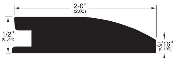
Reducer (090)
