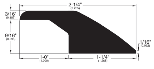
Reducer Overlap (035)
