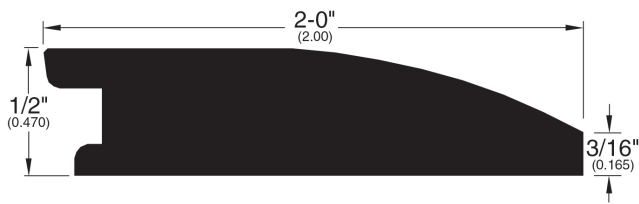
Reducer (010)
