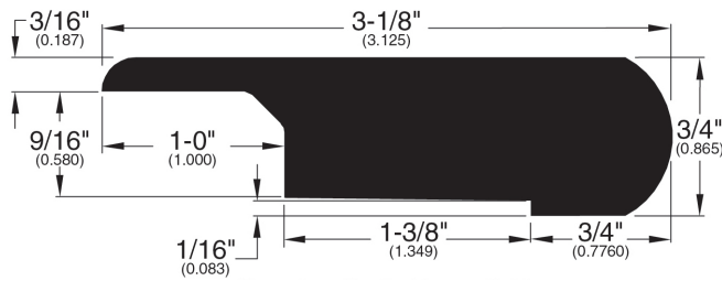
Stair Nose Overlap (036)
