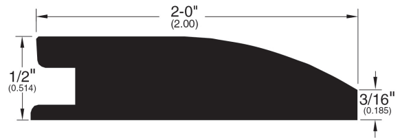
Reducer (090)
