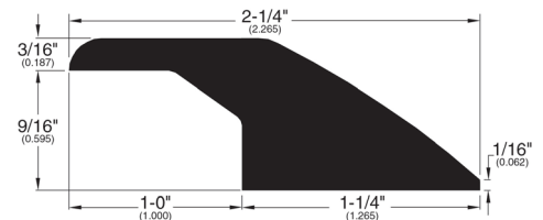
Reducer Overlap (035)
