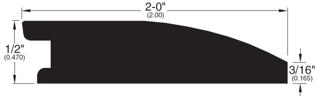
Reducer (010)
