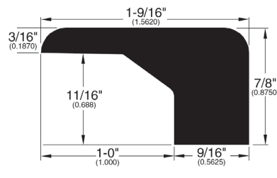
Square Nose (027)
