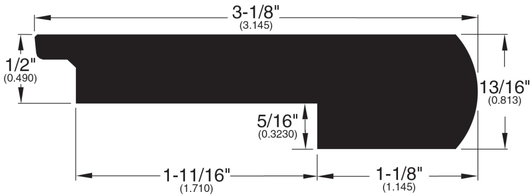
Stair Nose (067)
