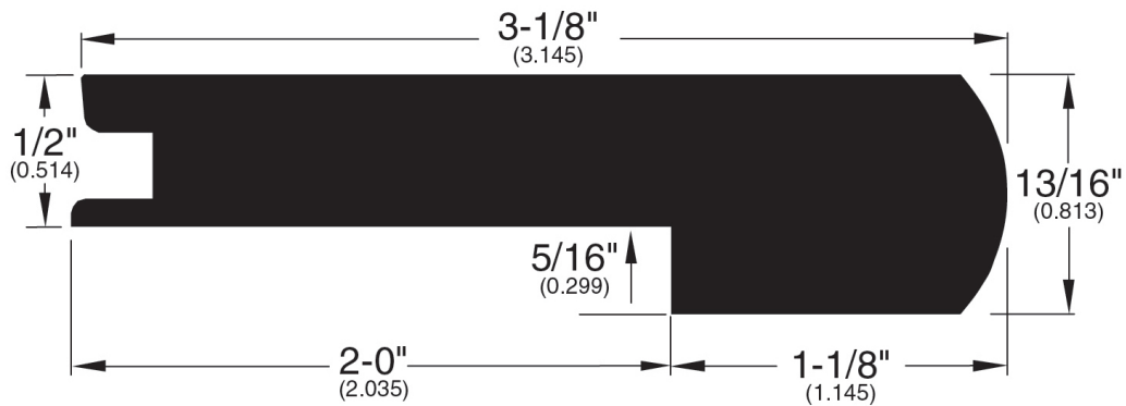
Stair Nose (091)
