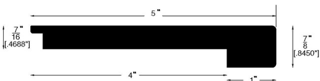
Sq Stair Nose (751)
