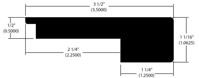
Square Stair Nose (714)
