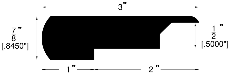
Stair Nose Overlap (745)
