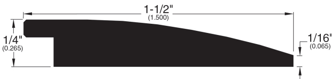
Reducer (022)
