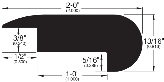
Stair Nose Overlap (030)
