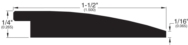
Reducer (022)
