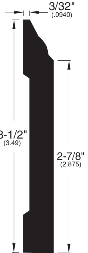
Reducer Overlap (029)
