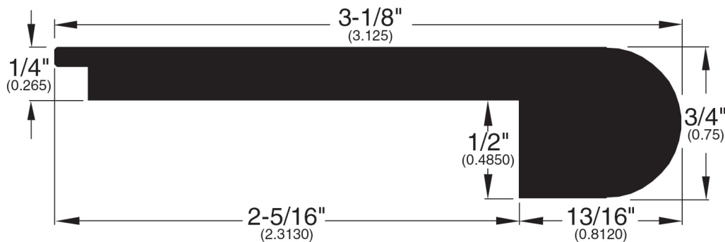
Stair Nose (023)
