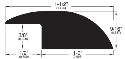
Reducer Overlap (029)
