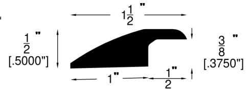
Reducer Overlap (747)
