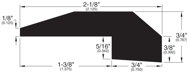
Threshold (008)
