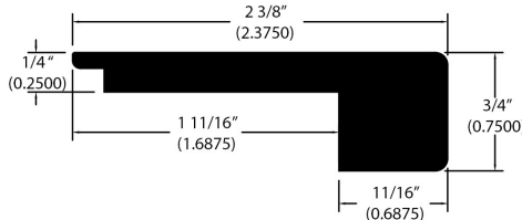
Square Stair Nose (724)
