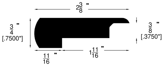
Stair Nose Overlap (744)
