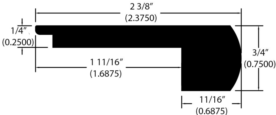
Stair Nose (723)
