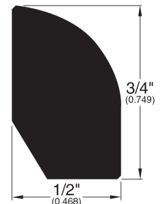
Base Shoe (024)
