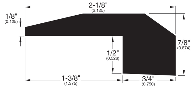
Threshold (011)
