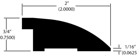
Reducer (716)
