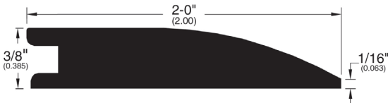
Reducer (007)
