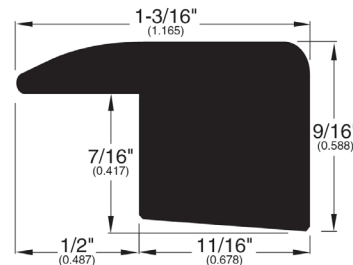
Square Nose (043)
