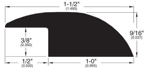
Reducer Overlap (029)
