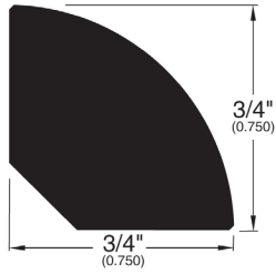
Quarter Round (001)
