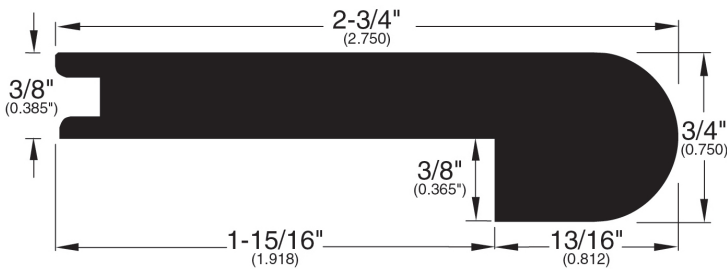
Stair Nose (009)
