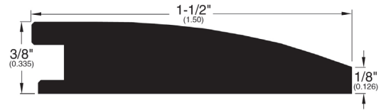
Reducer (018)
