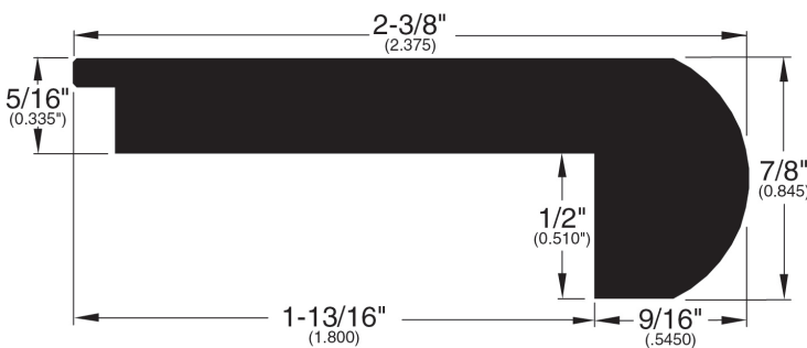
Stair Nose (019)
