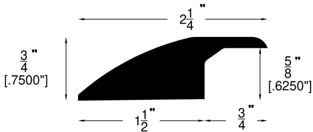
Reducer Overlap (749)
