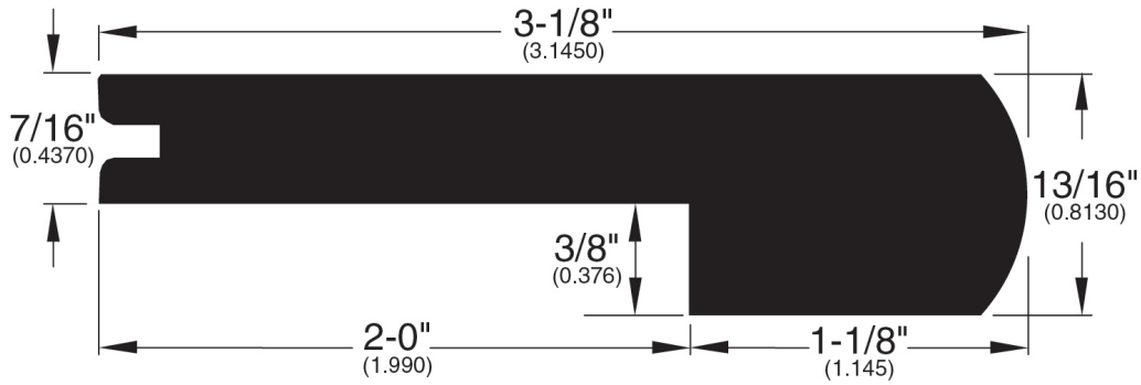
Stair Nose (057)
