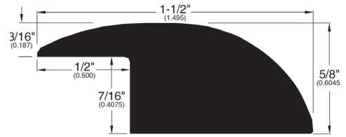
Reducer Overlap (095)
