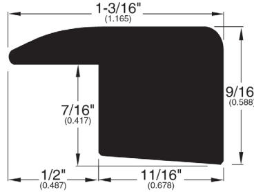
Square Nose (043)
