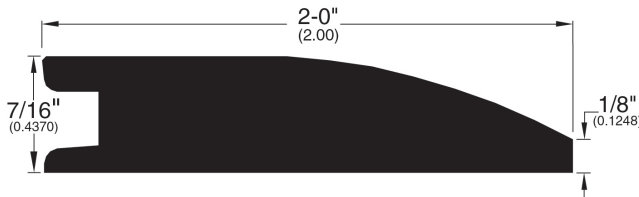
Reducer (041)
