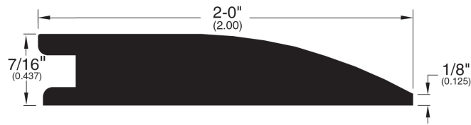
Reducer (056)
