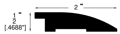
Reducer (710)
