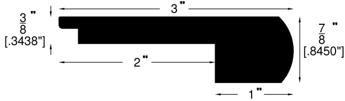
Stair Nose (709)
