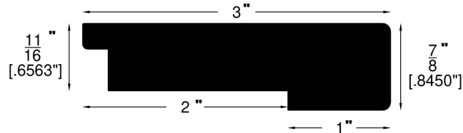
Stair Nose (782)
