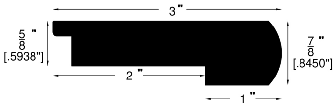
Stair Nose (738)
