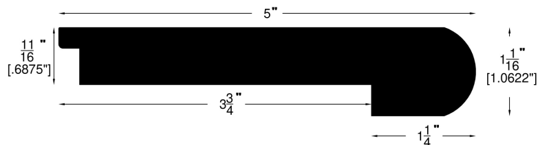
Stair Nose (054)
