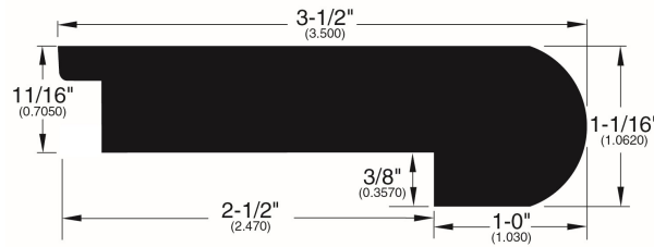
Stair Nose (761)
