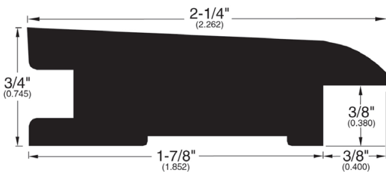
Reducer (045)
