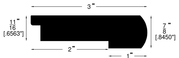
Stair Nose (781)
