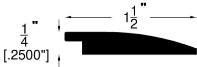
Reducer (722)
