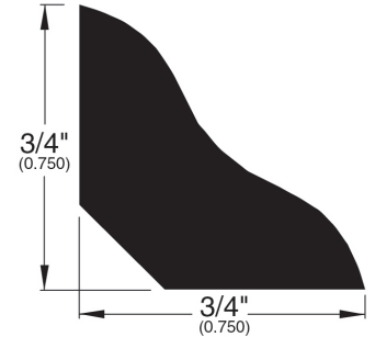
Cove (073)
