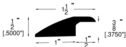
Reducer Overlap (747)
