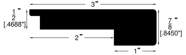
Stair Nose (713)
