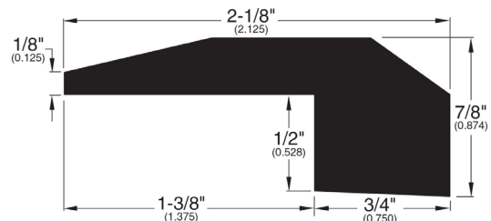
Threshold (011)
