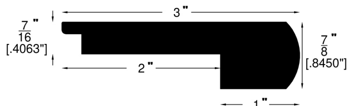
Stair Nose (742)
