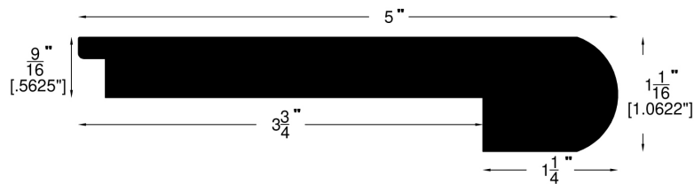
Stair Nose (154)
