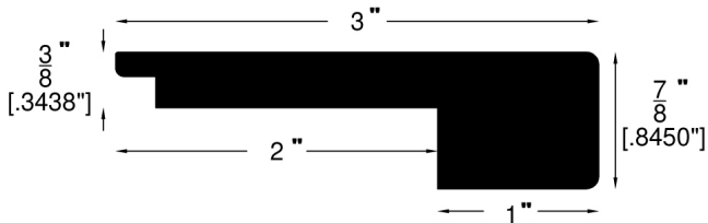
Stair Nose (718)
