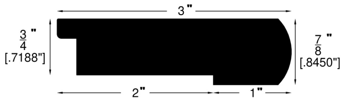
Stair Nose (717)
