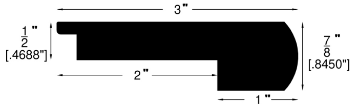
Stair Nose (712)
