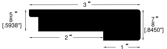
Stair Nose (739)
