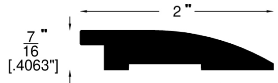
Reducer (741)
