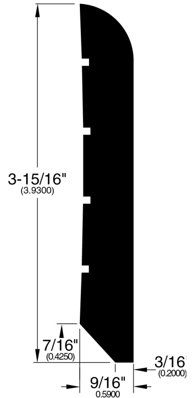
Wall Base (294)
