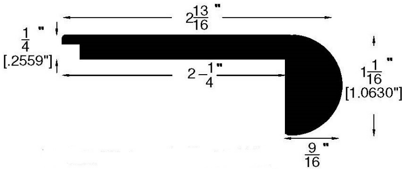
Stair Nose (288)
