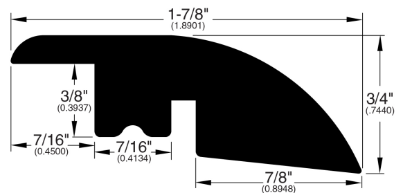
Overlap Reducer (293)
