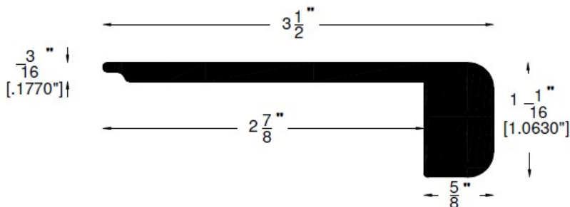
Stair Nose Square Edge (340)
