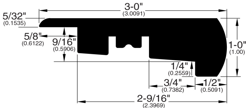
Overlap Stair Nose (292)
