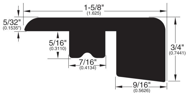
Square Nose (338)
