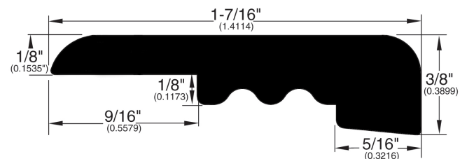
Square Nose (300)
