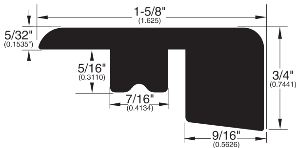
Square Nose (338)
