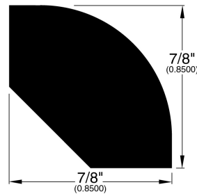
Quarter Round (296)
