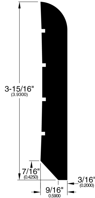
Wall Base (294)
