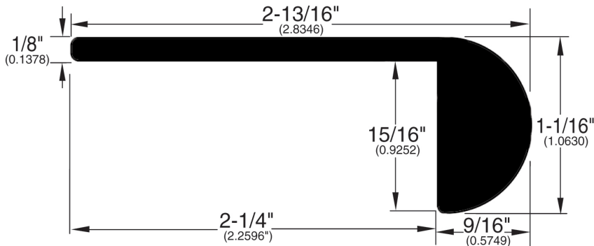
Stair Nose (298)
