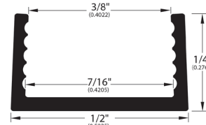
Track (286)
