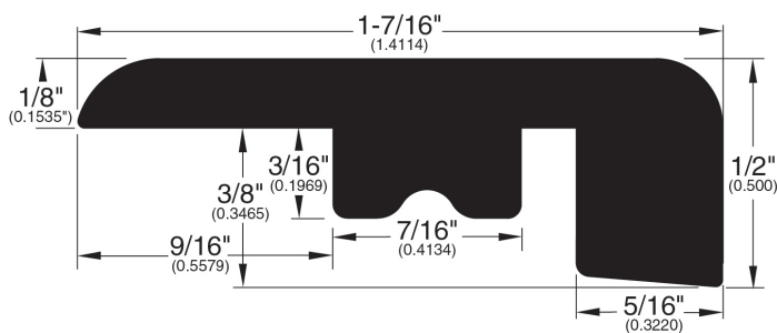
Square Nose (291)
