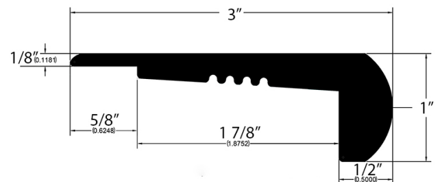
Stair Nose (273) *fits up to 6mm floors
