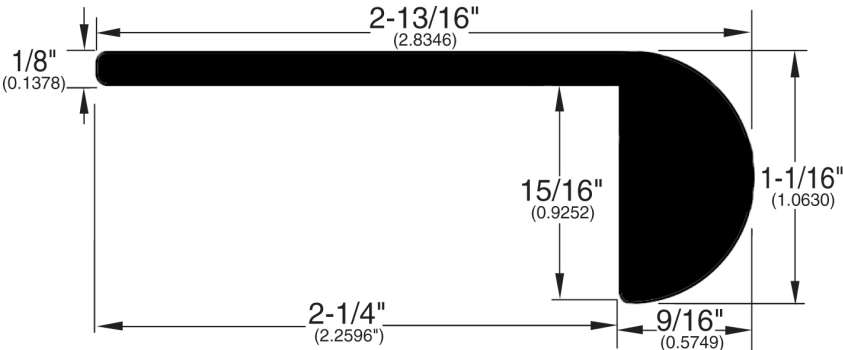
Stair Nose (298)
