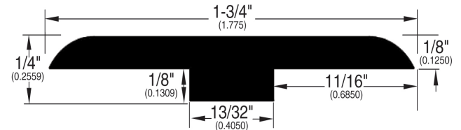
T-Mold (299) *fits up to 6mm floors
