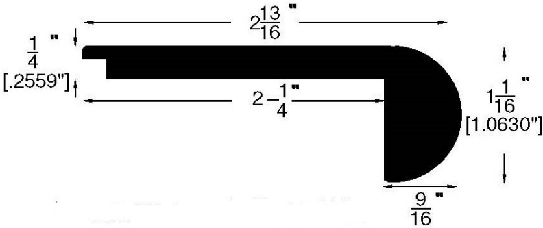
Stair Nose (288)
