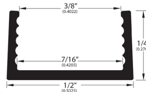
Track (286)
