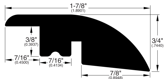
Overlap Reducer (293)
