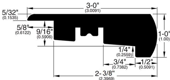
Enduracor Overlap Stair Nose (292)
