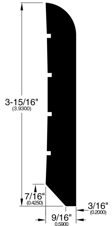
Wall Base (294)
