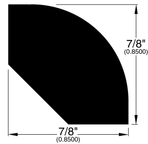
Quarter Round (296)
