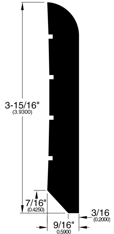
Wall Base (294)
