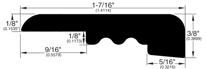
Square Nose (300)
