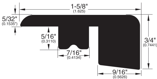
Square Nose (338)
