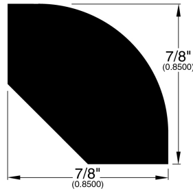
Quarter Round (296)
