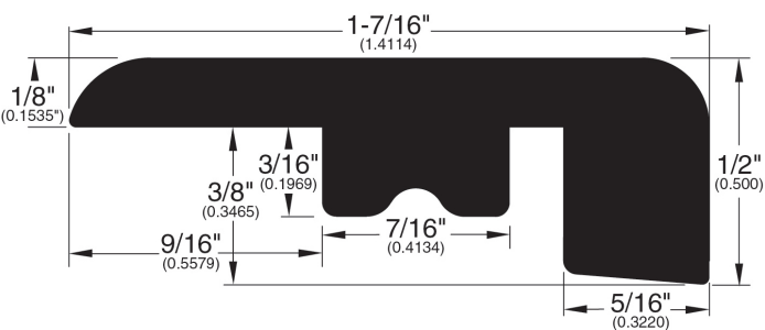
Square Nose (291)
