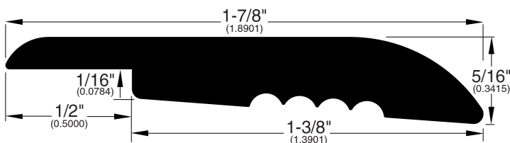
Overlap Reducer (297)
