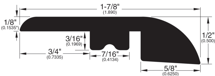
Overlap Reducer (290)
