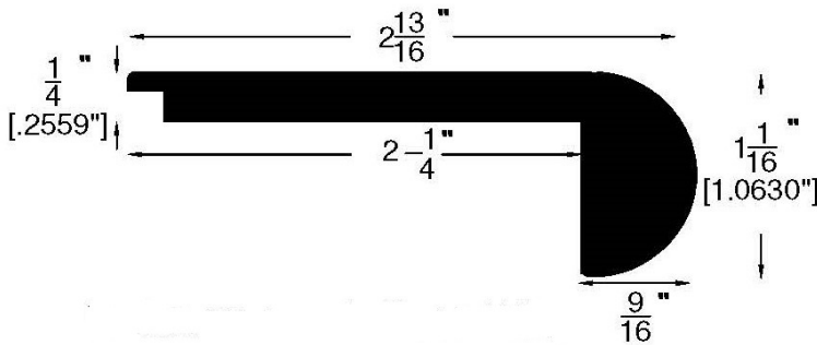
Stair Nose (288)*
