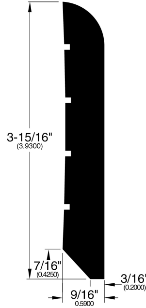
Wall Base (294)
