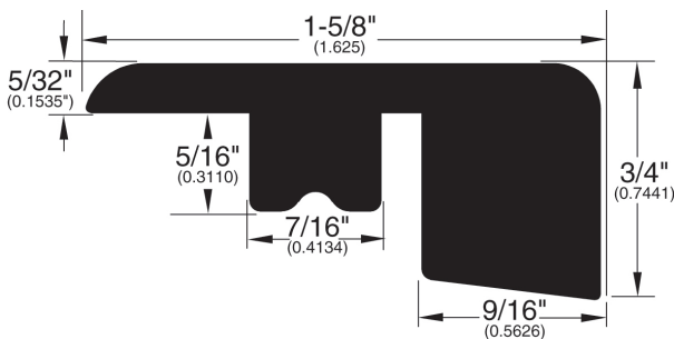
Square Nose (338)
