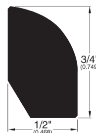
Base Shoe (024)
