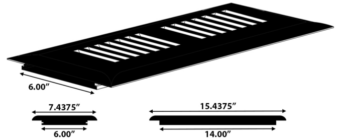
Surface Mount Vent 6" x 14"
